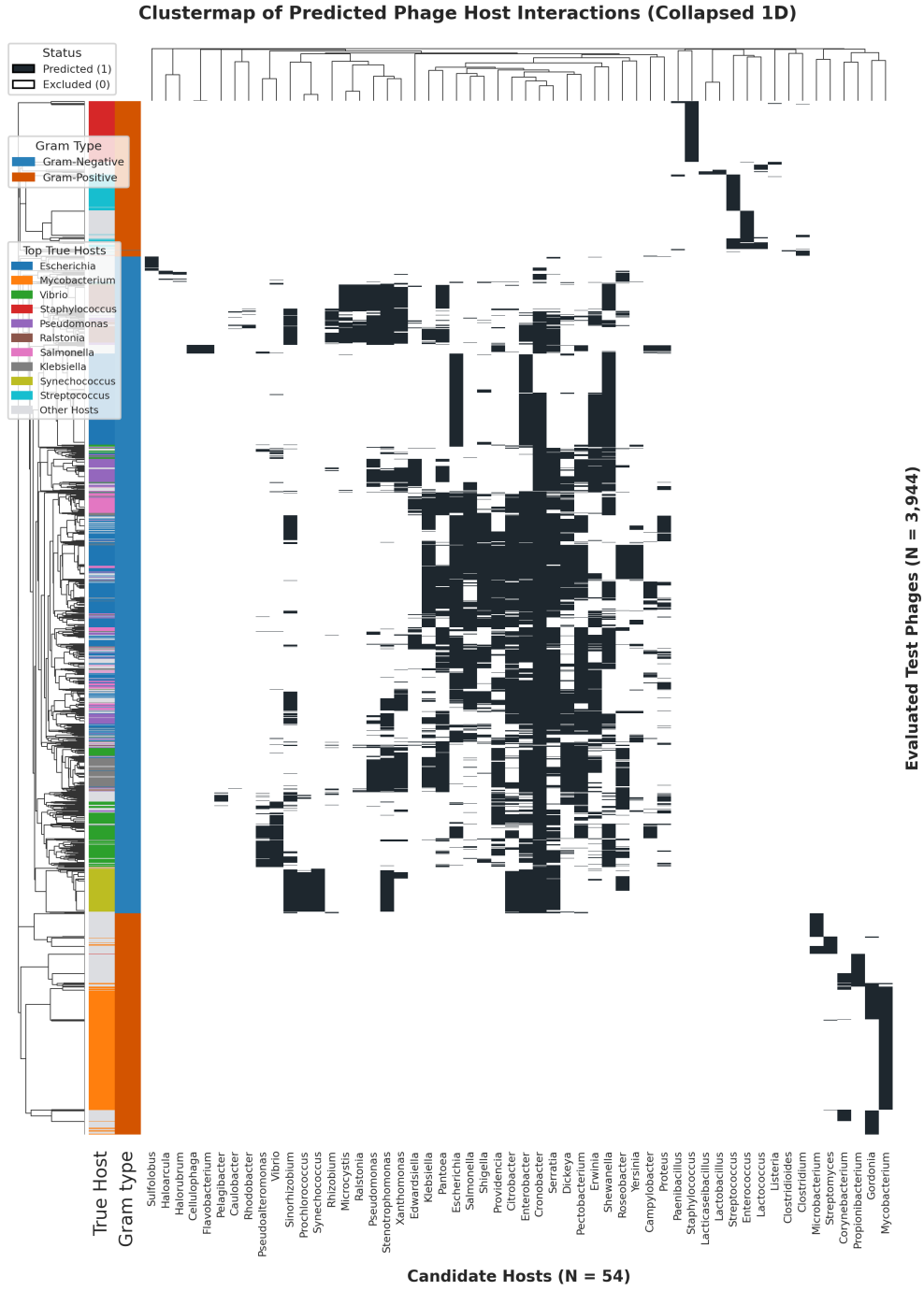
Figure 5.6: Clustermap of Predicted Phage Host Interactions (Collapsed 1D). Binary prediction matrix evaluated across all N_{\text{test}} = 3,944 test phages (rows) and 54 candidate host genera (columns) under the Collapsed 1D method ( 1 - \alpha = 0.90 ). Dark pixels denote host inclusion in the conformal prediction set C(s) . Left sidebars indicate ground-truth Gram phenotype (blue: Gram-negative, orange: Gram-positive) and top true host genera.
